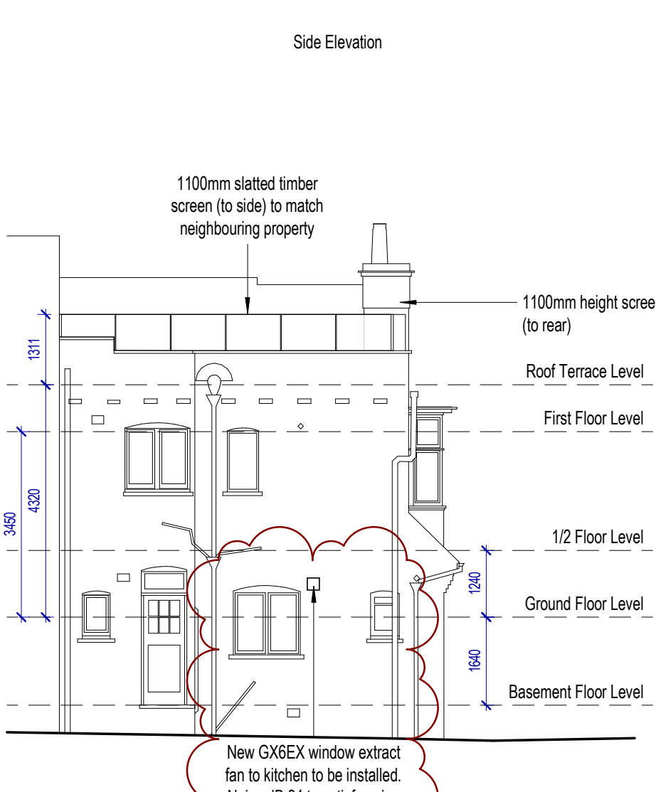
3 Side Elevation Proposed PP104 1 : 100
