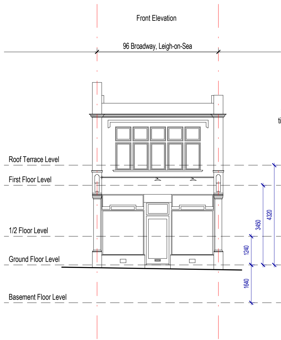
1 Front Elevation Proposed PP104 1 : 100
