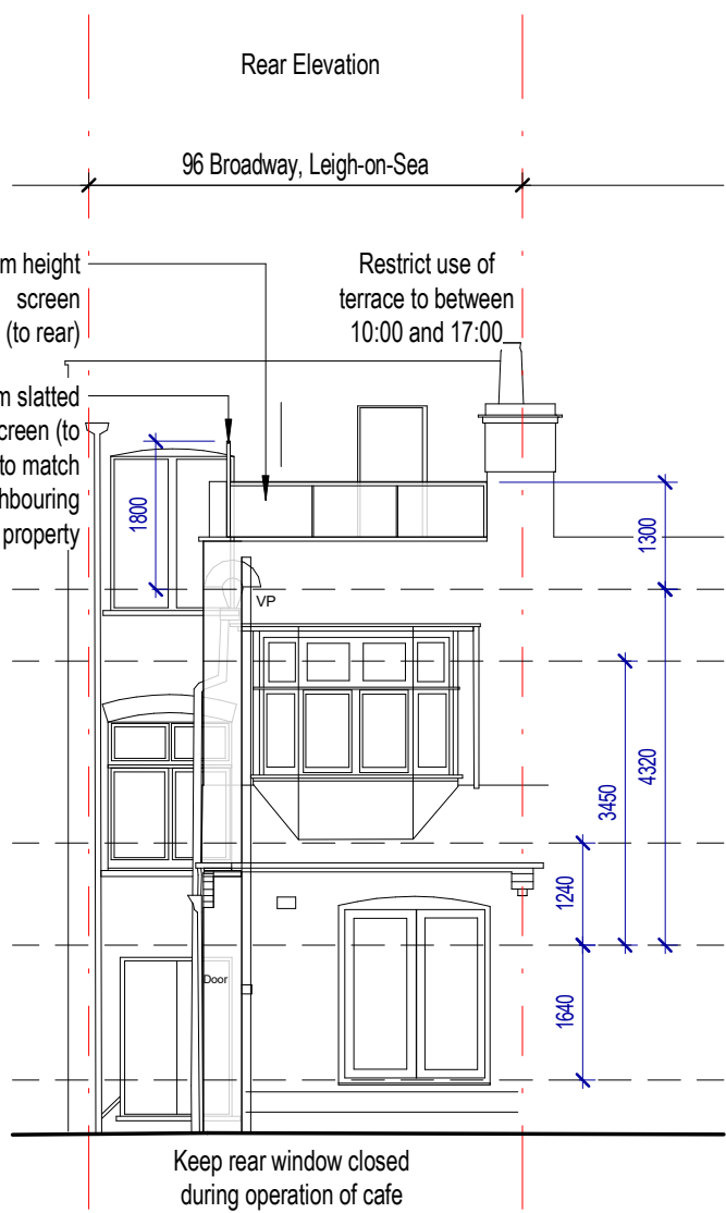
2 Rear Elevation Proposed PP104 1 : 100
